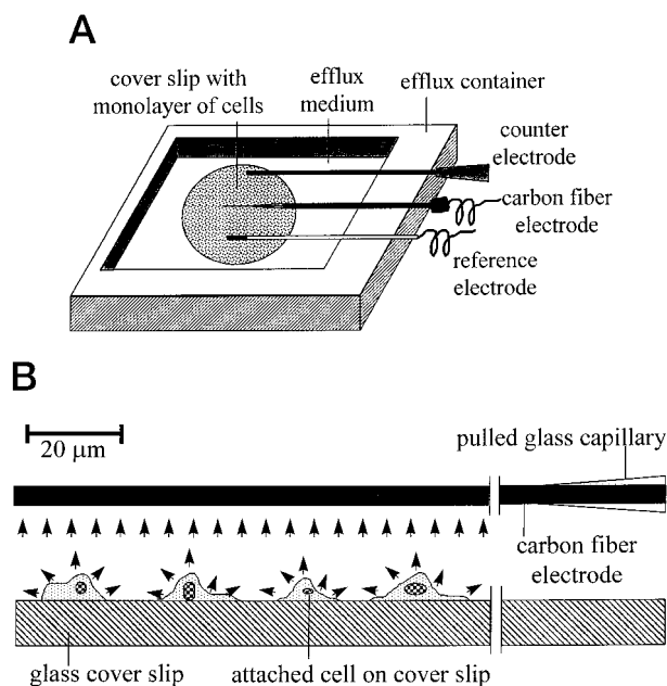
FIGURE 1 Experimental arrangement for doxorubicin efflux measurements. (A) The efflux container, made of plexiglas and covered by a plastic cover ensuring free air exchange between inside and outside the covered space (the cover is not shown here). The glass coverslip and the electrodes are under the efflux medium. The depth of the medium is \sim 1 mm. The electrodes are placed horizontally side by side, and the CF electrode is in the middle. The diameter of the coverslip is 4 cm. (B) Enlarged schematic diagram of the relative positions of the carbon fiber electrode and the effluxing cells. The arrows show the directions and patterns of diffusion of the effluxed doxorubicin.
